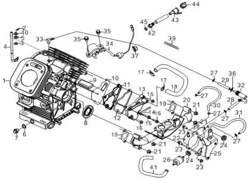
FIG.1 CRANKCASE/GOVERNOR GEAR ASSEMBLY
