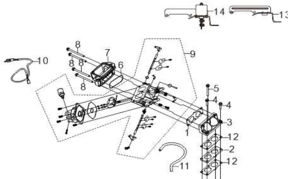
FIG.8 CARBURETOR ASSEMBLY
