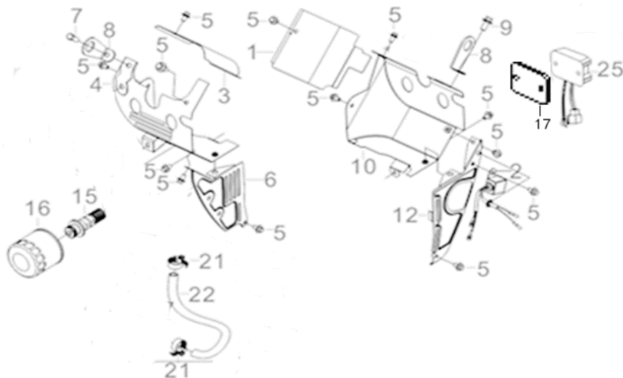
FIG.7 SHROUD
