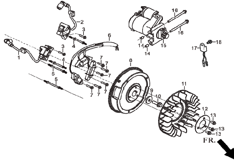
FIG.9 FLYWHEEL / IMPELLER / STARTER PULLEY / IGNITION COIL
