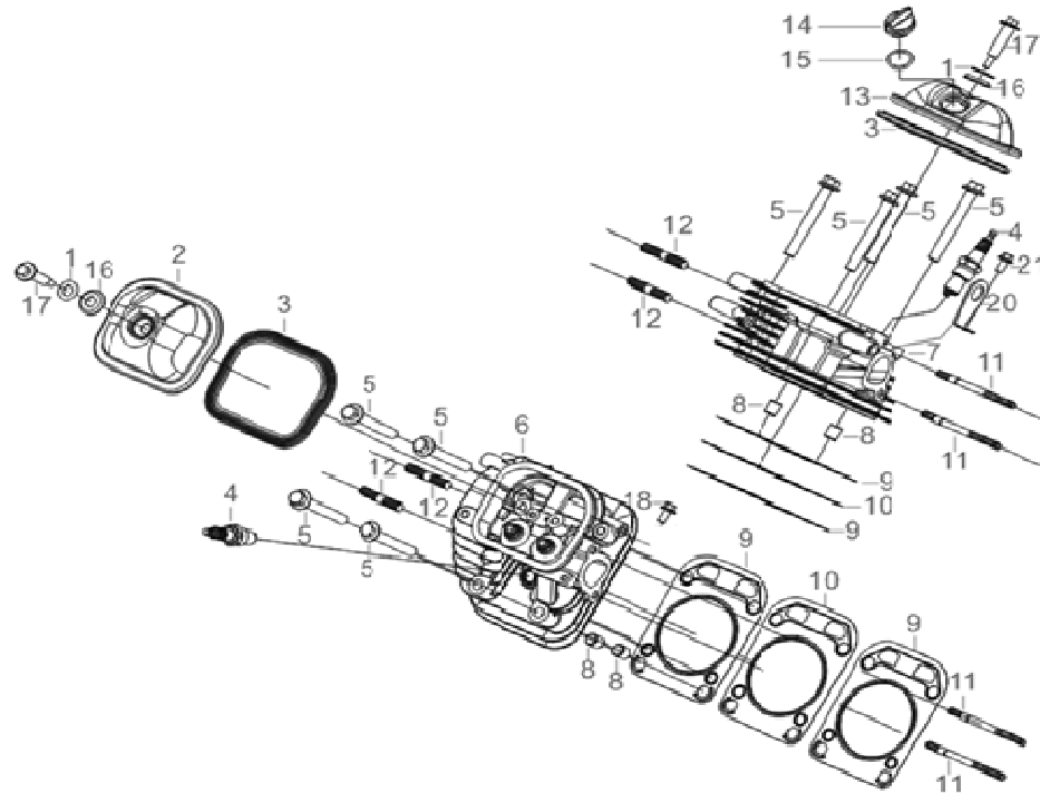
FIG.3 SPARK PLUG,CYLINDER HEAD SUBASSEMBLY
