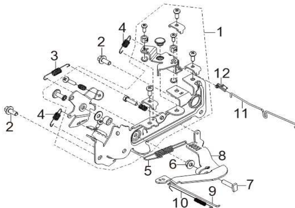
FIG.10 THROTTLE CONTROL ASSEMBLY
