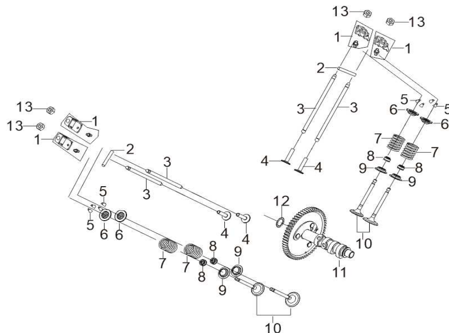
FIG.5 TRAIN VALVE / CAMSHAFT SUBASSEMBLY
